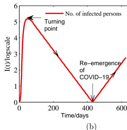
Fig. 6. (a) The number of infected persons as a function of time to linear scale. (b) The number of infected persons as a function of time to logarithm scale for R_{n0} = 0.46
